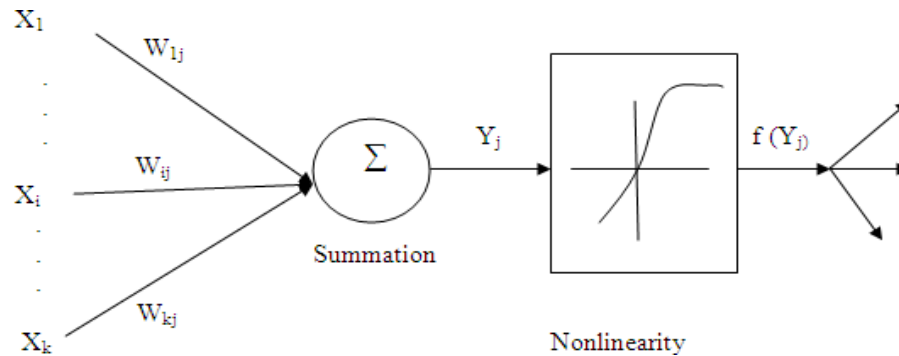
Figure: 4 ANN modelling for Hypervisor Scanner
